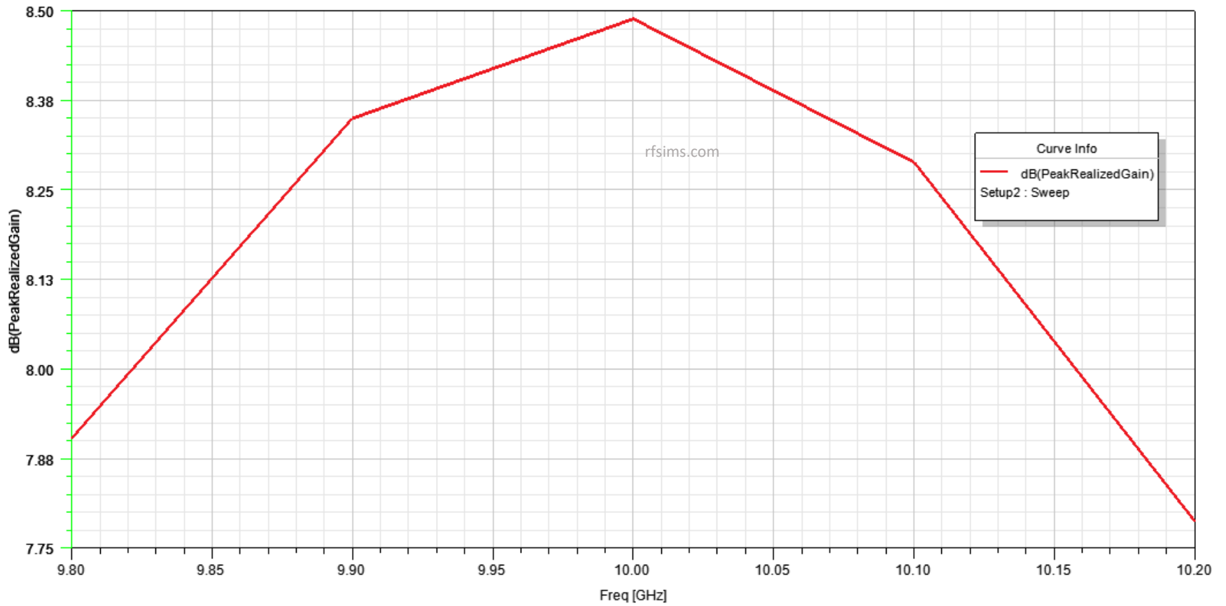
Peak Realized Gain (dBi) vs Frequency (GHz)
