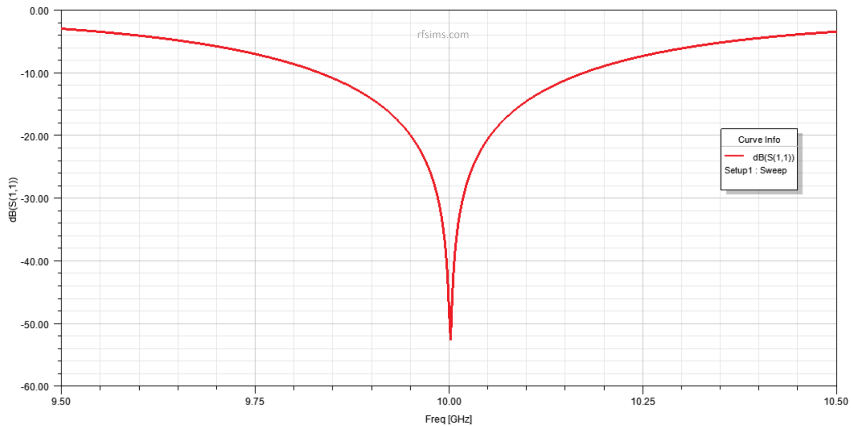
Return Loss (dB) vs Frequency (GHz)
