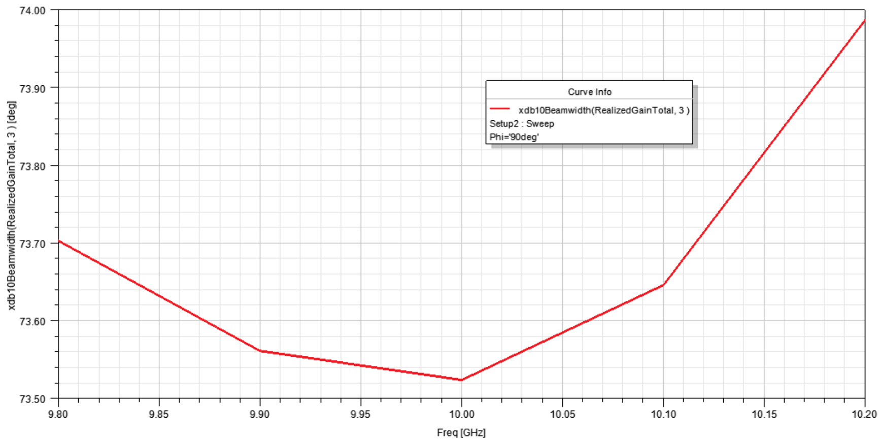
H-Plane Beamwidth (deg) vs Frequency (GHz)
