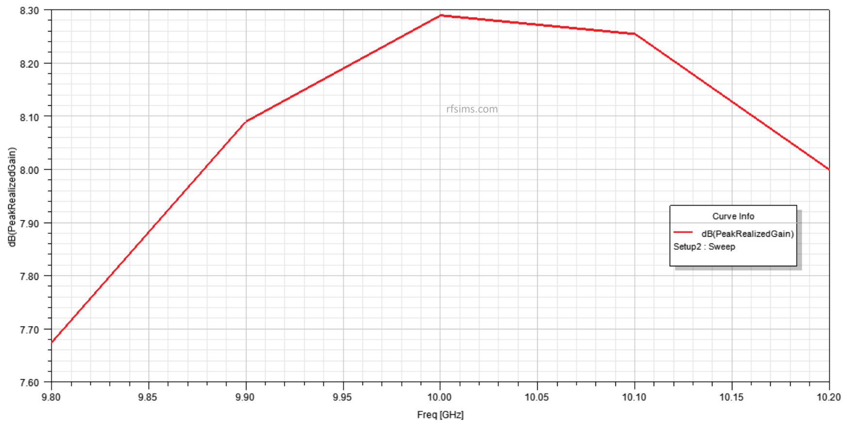
Peak Realized Gain (dBi) vs Frequency (GHz)
