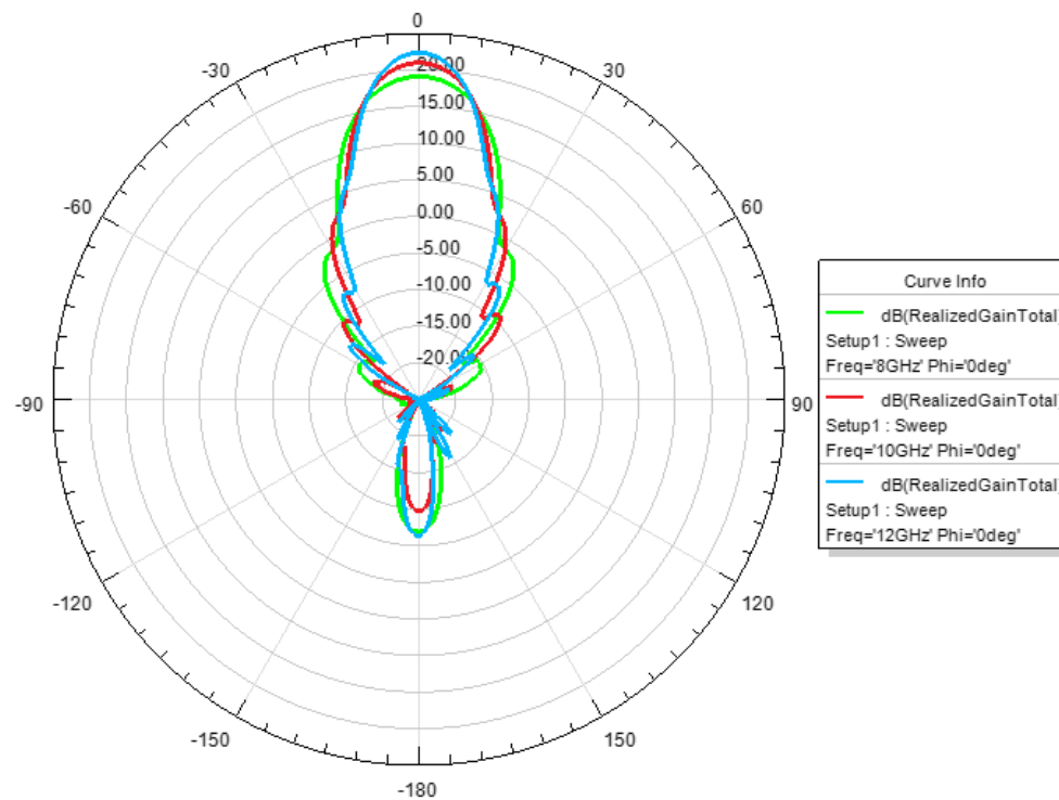
H-Plane Total Realized Gain (dBi) vs Angle (deg)
