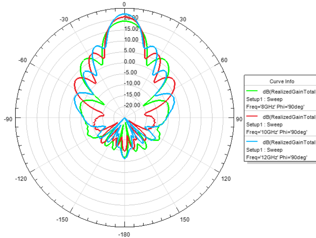
E-Plane Total Realized Gain (dBi) vs Angle (deg)
